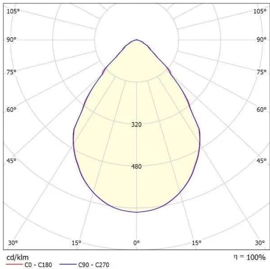
Photometric drawing
