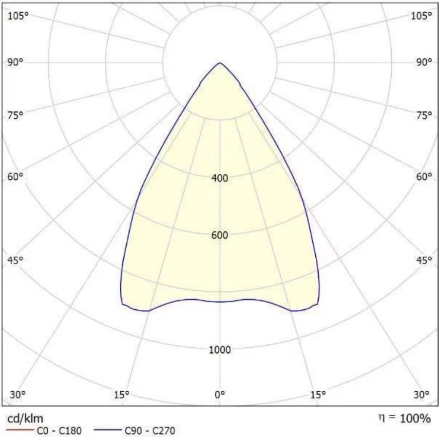
Photometric drawing
