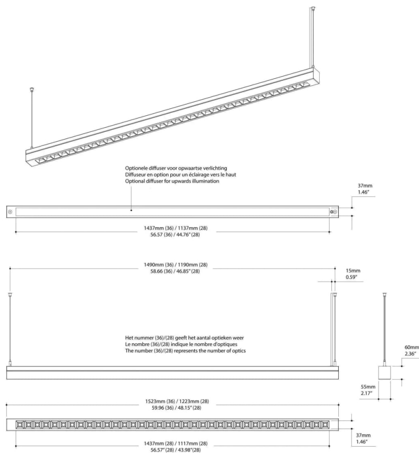
Photometric drawing
